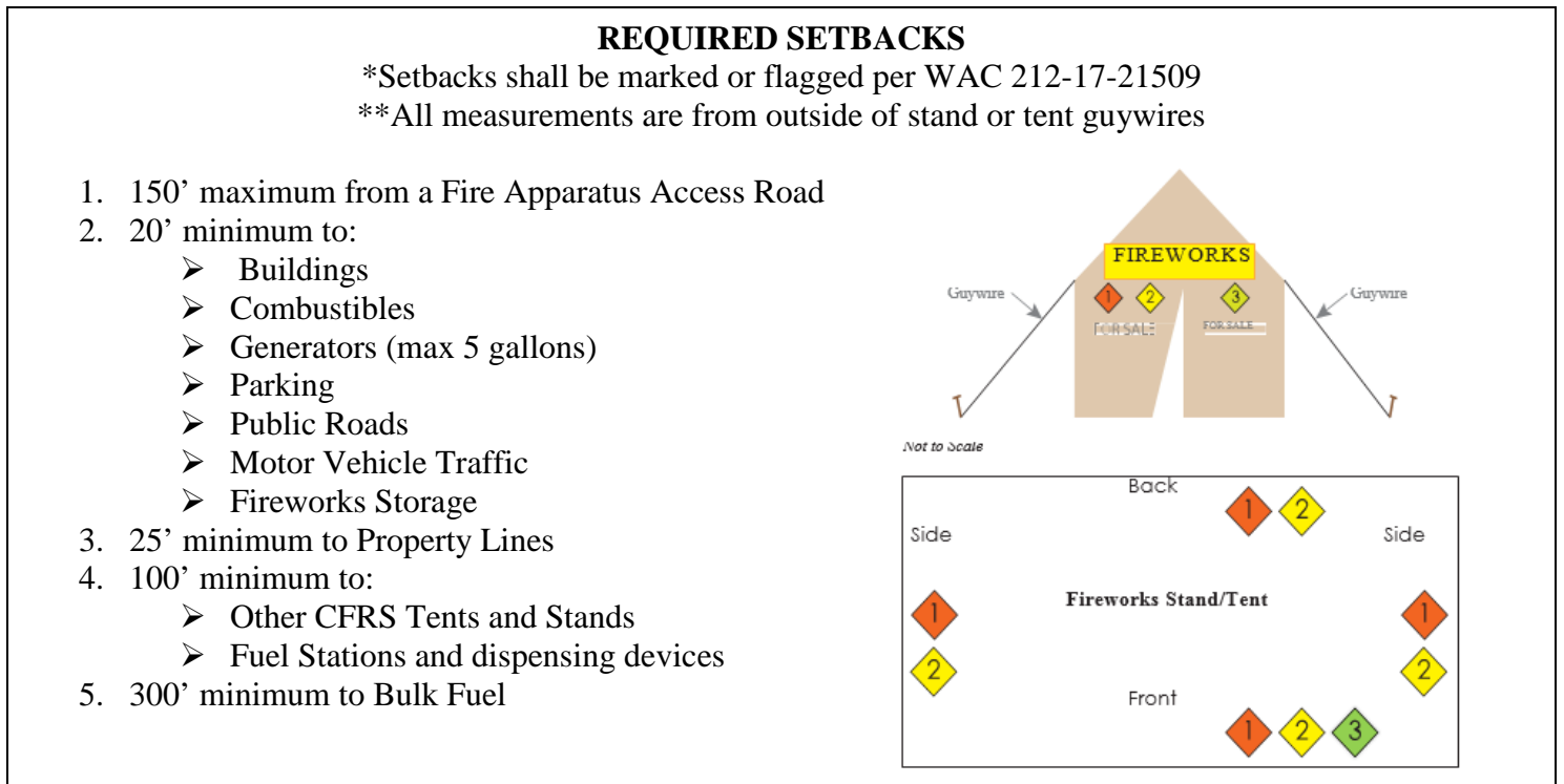
Figure 1: Required Setbacks
